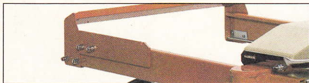
Locking mechanism for press unit in rear position.
